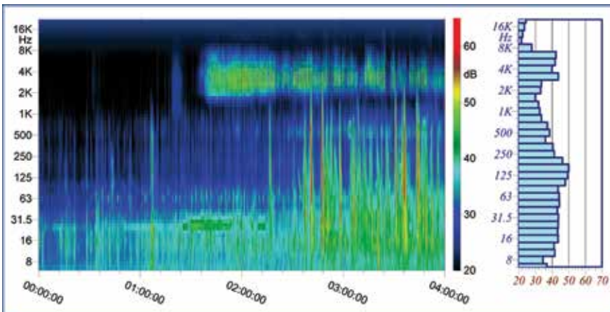
Spectrogram of Events with High Frequency Noise
