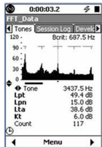
Model 831 Tonality Calculation
