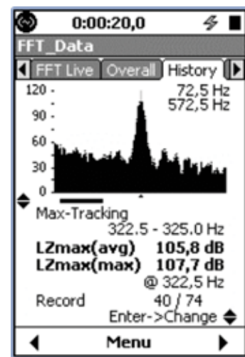
FFT Max-tracking on Model 831
