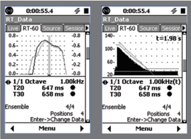
RT Displays of Decay Curves
